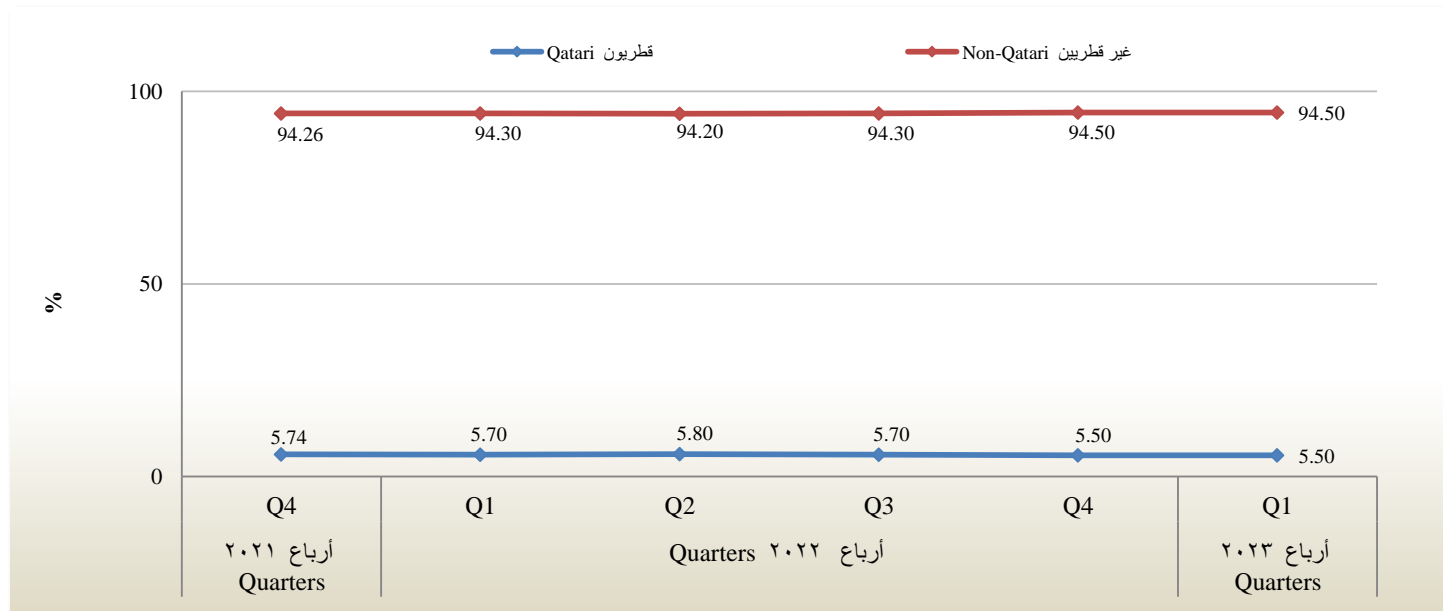
Figure 2 / Relative Evolution of the Economically Active by Nationality, during (Q4 2021 .. Q1 2023)
