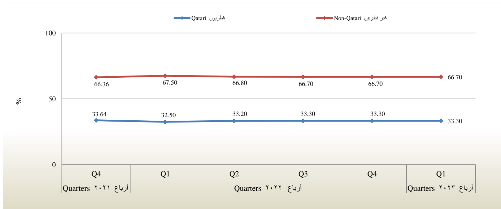
Figure 3 / Relative Evolution of the Economically Inactive by Nationality ( Qatari , Non-Qatari ), during (Q4 2021 .. Q1 2023)
